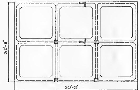
SECTION E-E. PLAN OF TOP OF BIN WALLS
